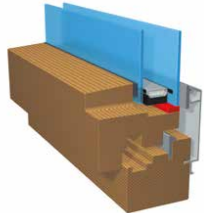
Glass Edge Bonding with Sikasil® WT Technology
